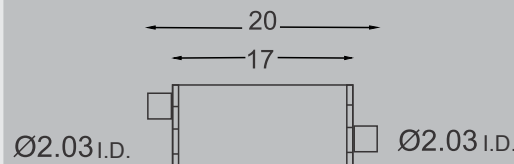
PART #AM-1787 CROSS SECTION 4 1/2" X 9 3/4"
