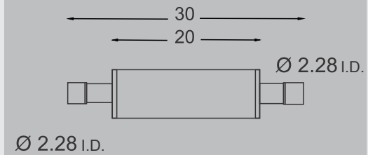
PART #AM-1794/5794 CROSS SECTION 6"
