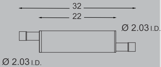
PART #AM-1785/2785 CROSS SECTION 6"
