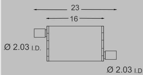
PART #AM-1780/9780 CROSS SECTION 4 1/2" X 9 3/4"
