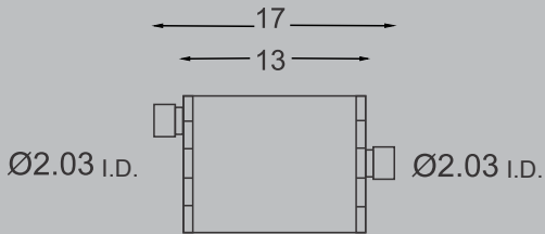
PART #AM-1779 CROSS SECTION 4 1/2" X 9 3/4"
