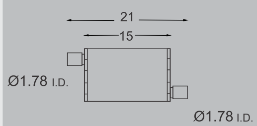
PART #AM-1783/5783 CROSS SECTION 4 1/2" X 9 3/4"
